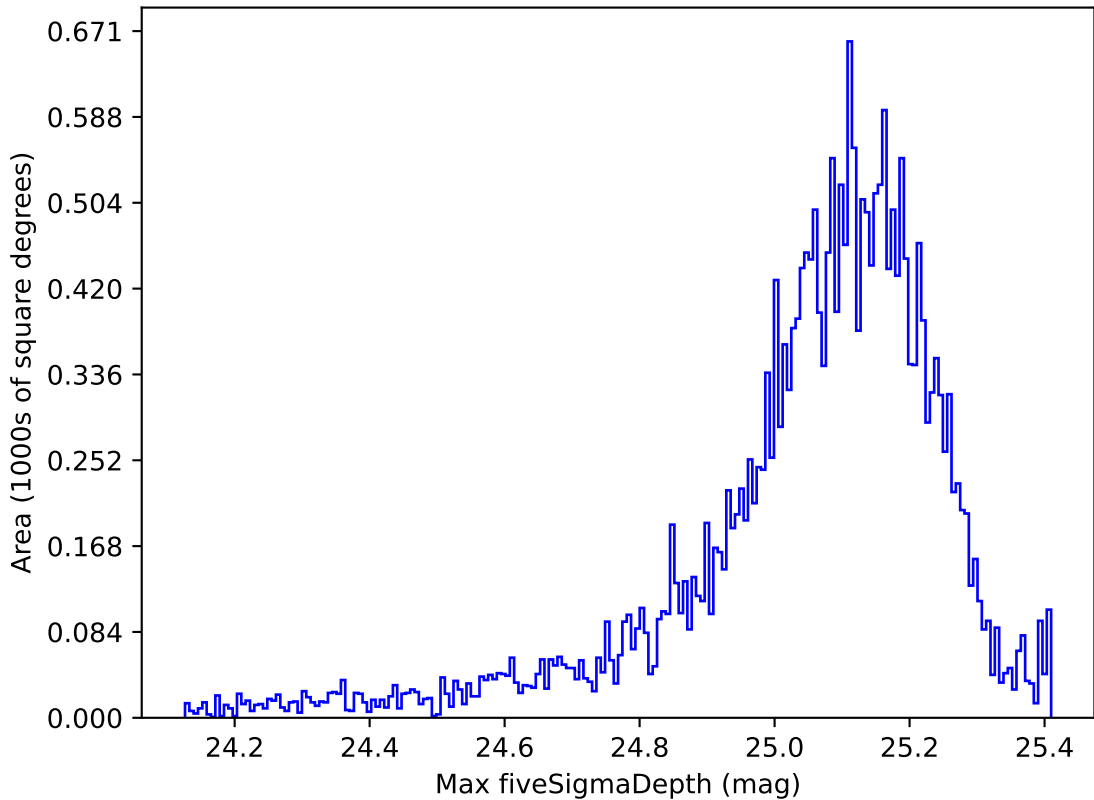
noroll_mjdp270_v3.4_10yrs All sky all bands: Max fiveSigmaDepth
