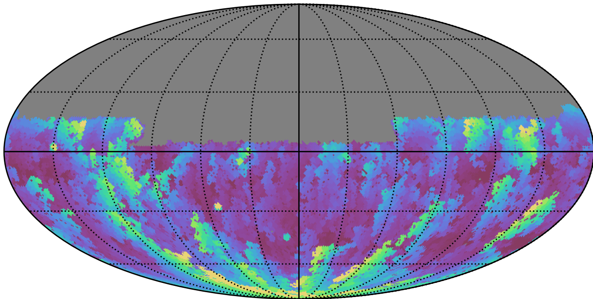
noroll_mjdp270_v3.4_10yrs Yr 1 u band: Max airmass
