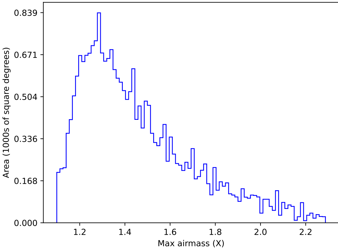
noroll_mjdp270_v3.4_10yrs Yr 1 u band: Max airmass
