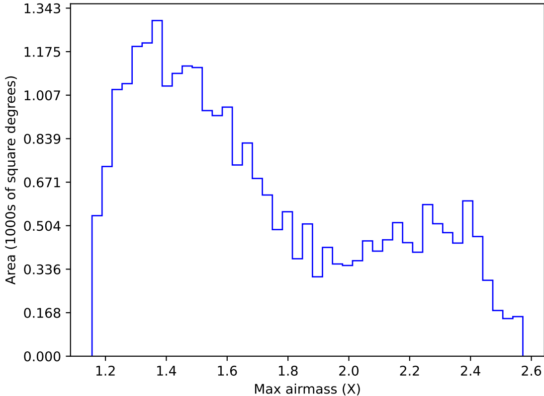
noroll_mjdp270_v3.4_10yrs Yr 1 r band: Max airmass
