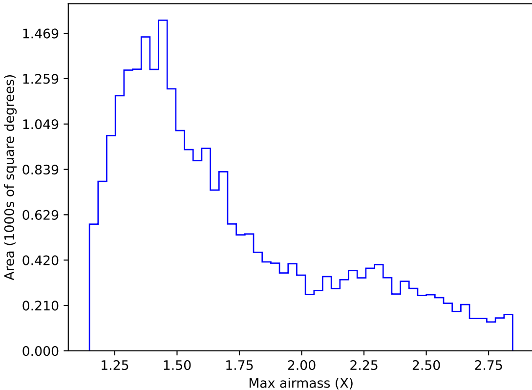
noroll_mjdp270_v3.4_10yrs Yr 1 i band: Max airmass
