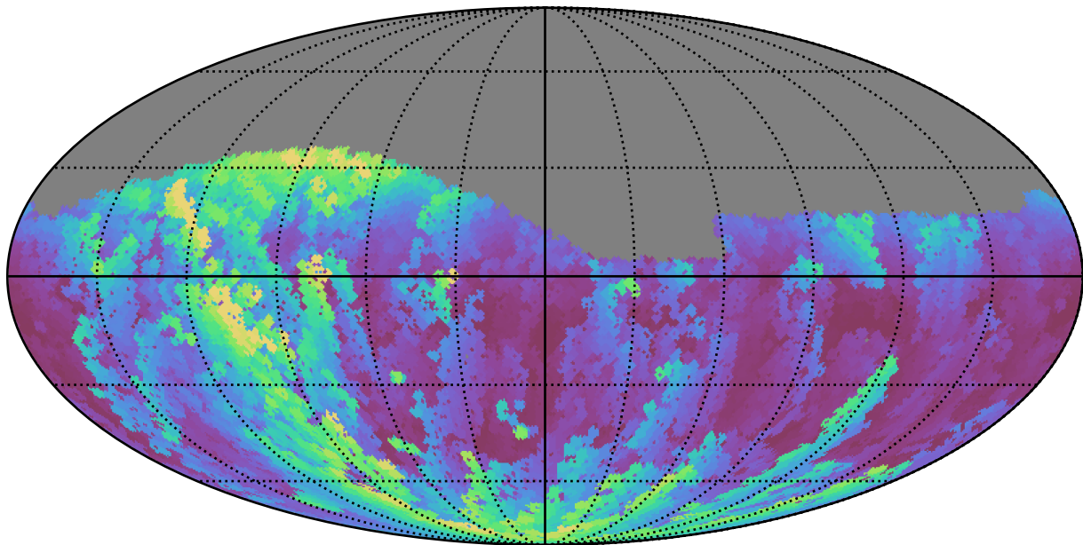
noroll_mjdp270_v3.4_10yrs Yr 1 g band: Max airmass
