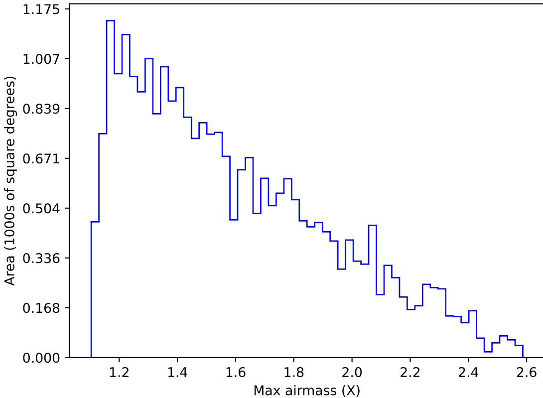
noroll_mjdp270_v3.4_10yrs Yr 1 g band: Max airmass
