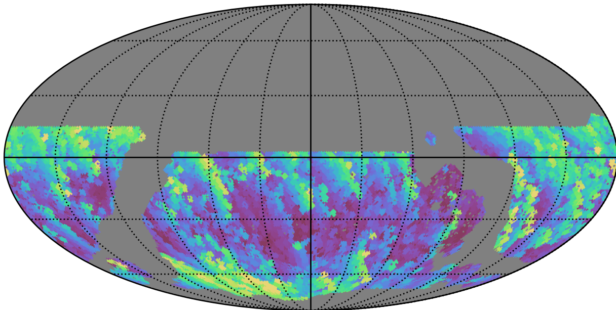
noroll_mjdp270_v3.4_10yrs WFD y band: Max airmass
