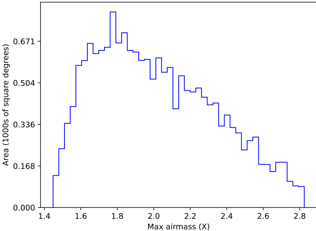
noroll_mjdp270_v3.4_10yrs WFD y band: Max airmass
