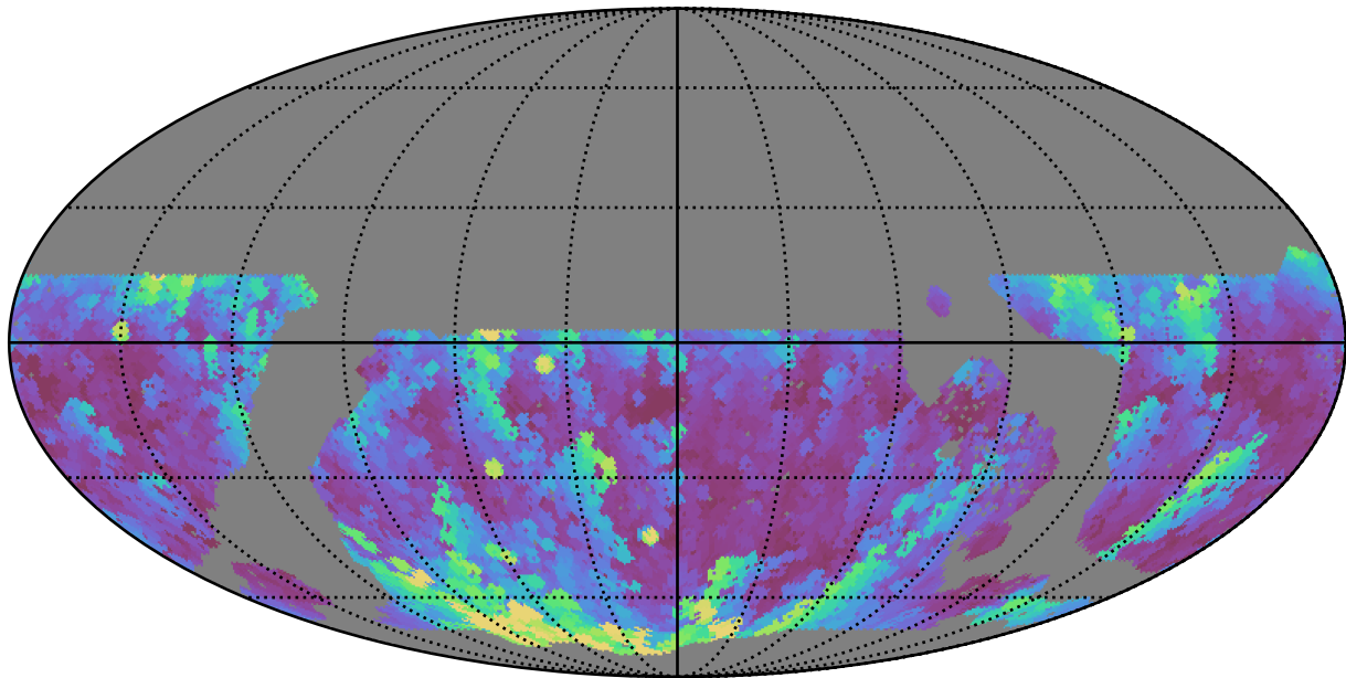
noroll_mjdp270_v3.4_10yrs WFD u band: Max airmass
