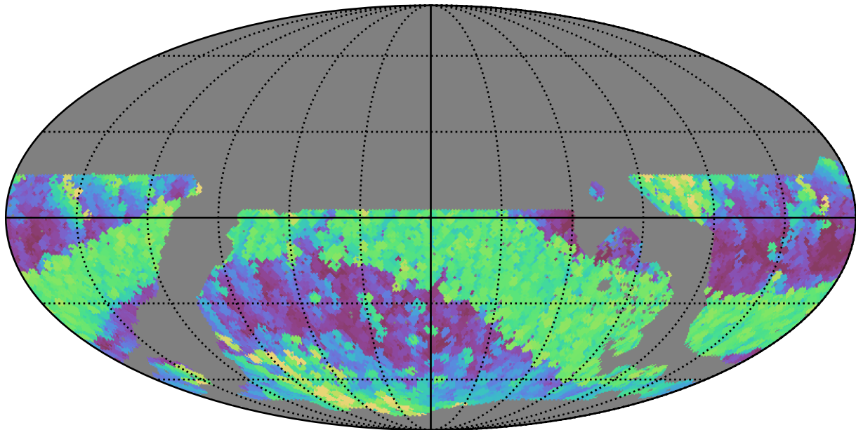
noroll_mjdp270_v3.4_10yrs WFD r band: Max airmass
