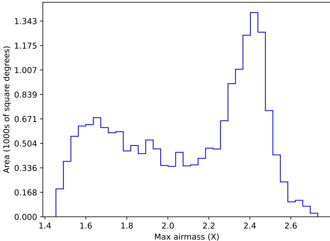
noroll_mjdp270_v3.4_10yrs WFD r band: Max airmass
