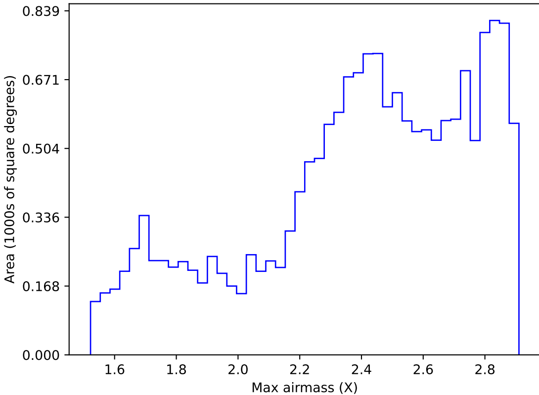
noroll_mjdp270_v3.4_10yrs WFD i band: Max airmass
