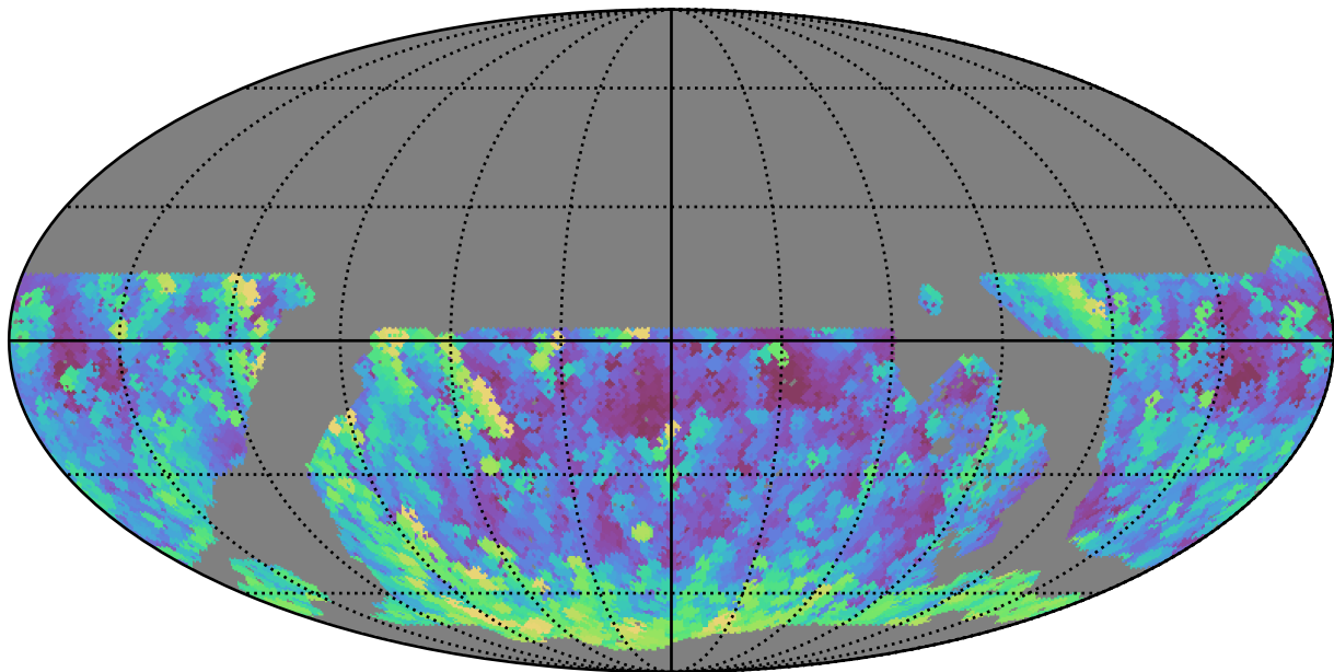
noroll_mjdp270_v3.4_10yrs WFD g band: Max airmass
