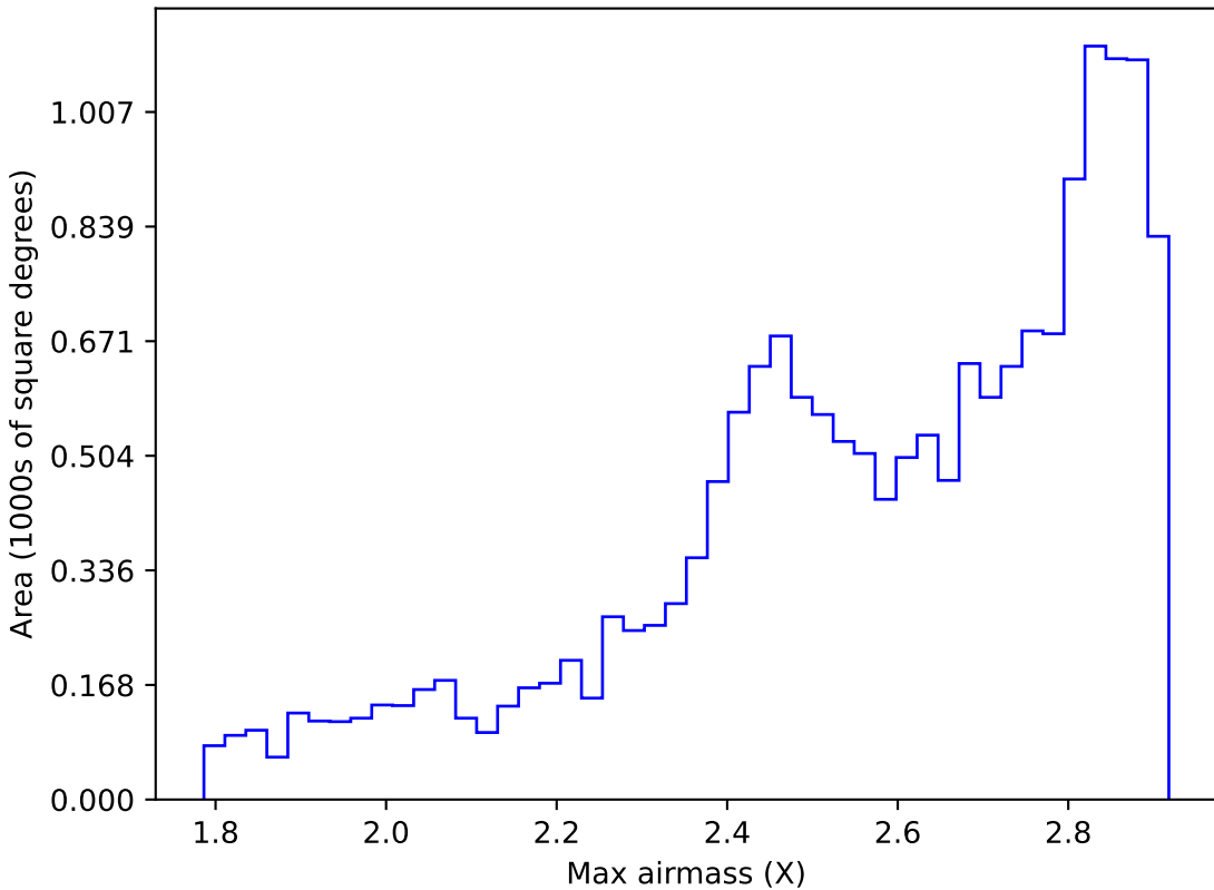
noroll_mjdp270_v3.4_10yrs WFD all bands: Max airmass
