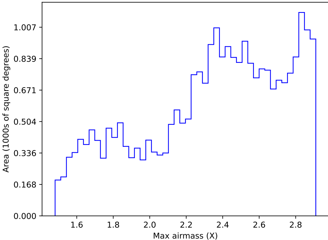
noroll_mjdp270_v3.4_10yrs All sky z band: Max airmass
