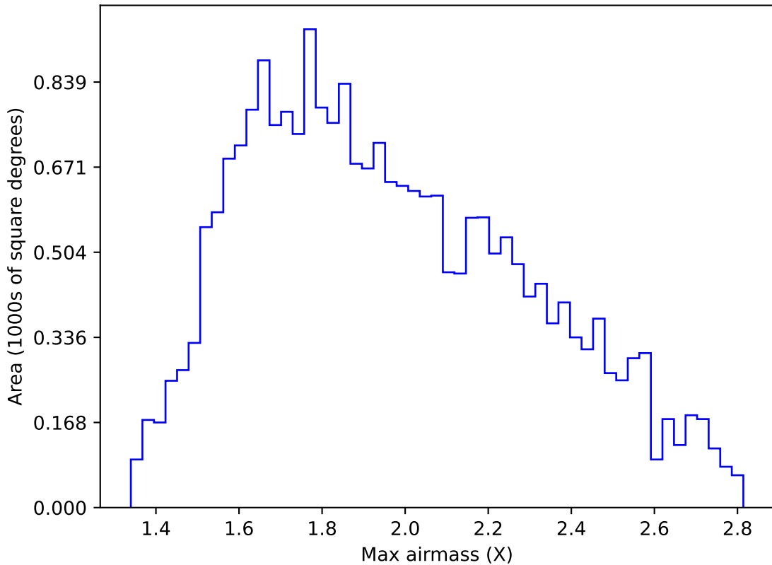
noroll_mjdp270_v3.4_10yrs All sky y band: Max airmass
