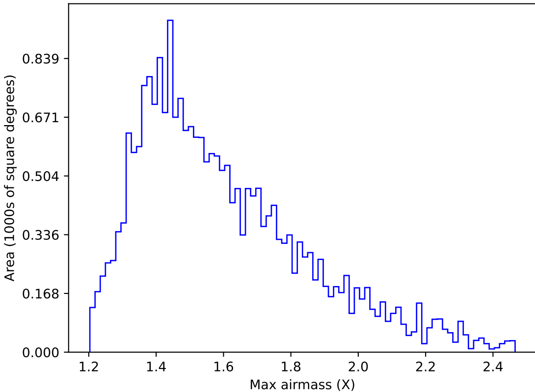
noroll_mjdp270_v3.4_10yrs All sky u band: Max airmass
