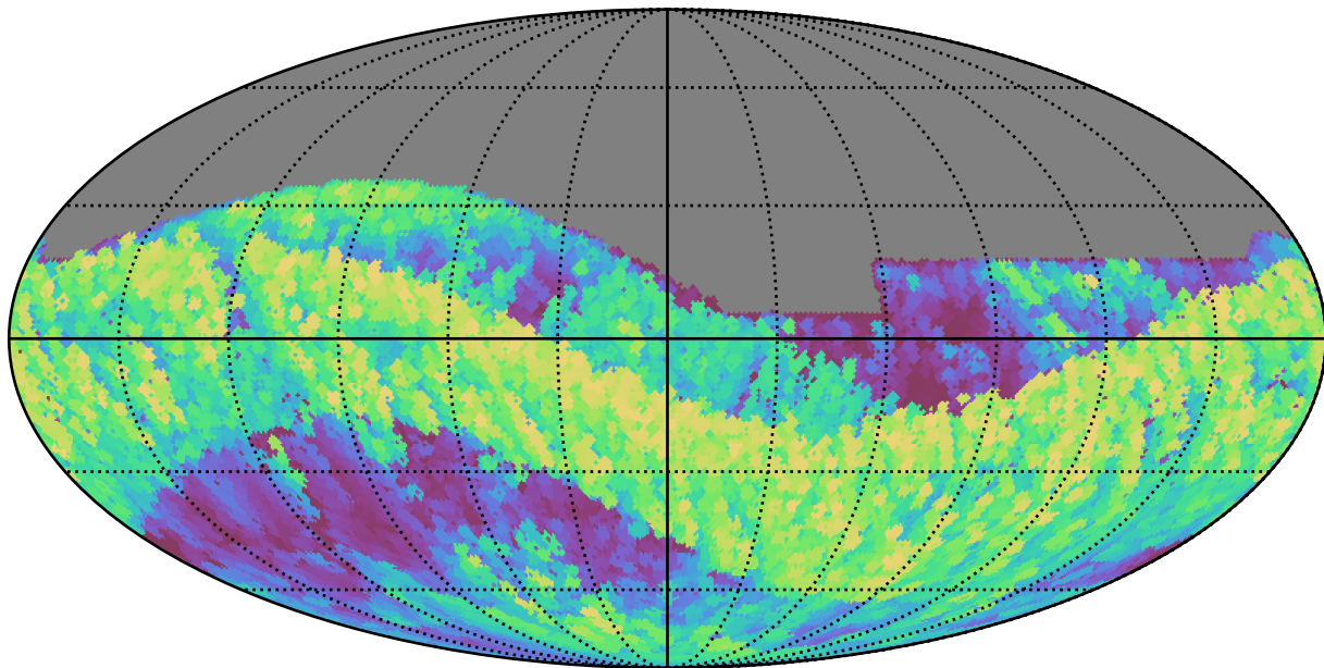
noroll_mjdp270_v3.4_10yrs All sky i band: Max airmass
