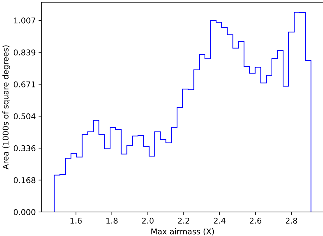
noroll_mjdp270_v3.4_10yrs All sky i band: Max airmass
