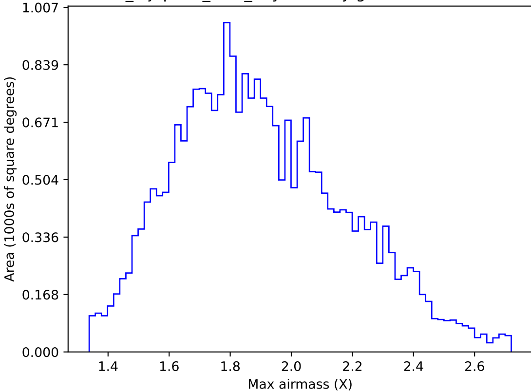
noroll_mjdp270_v3.4_10yrs All sky g band: Max airmass
