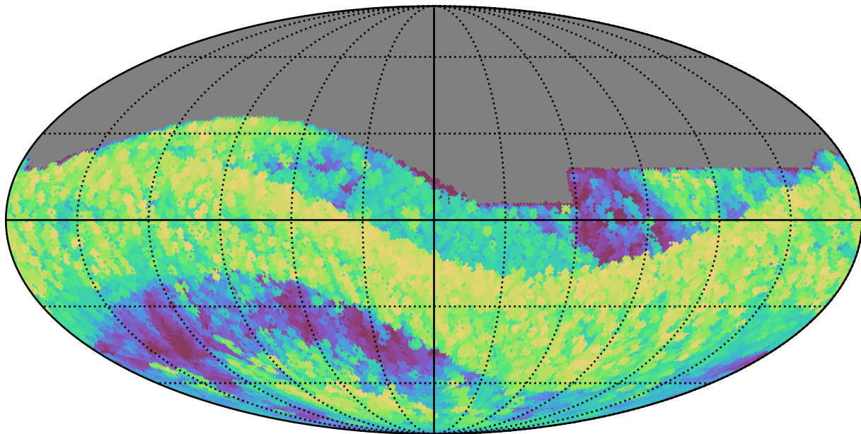
noroll_mjdp270_v3.4_10yrs All sky all bands: Max airmass
