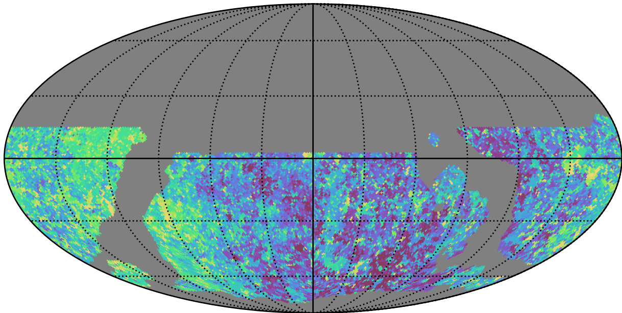
noroll_mjdp270_v3.4_10yrs WFD z band: Max Inter-Night Gap
