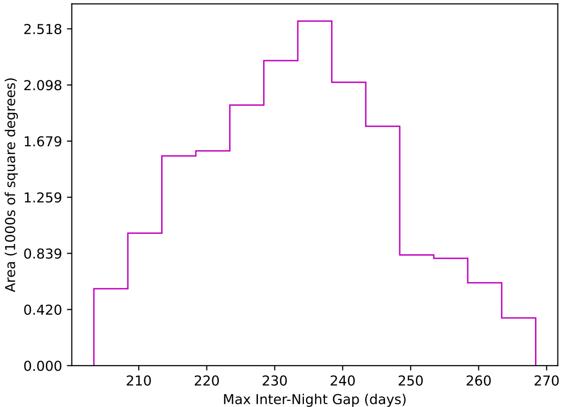
noroll_mjdp270_v3.4_10yrs WFD z band: Max Inter-Night Gap
