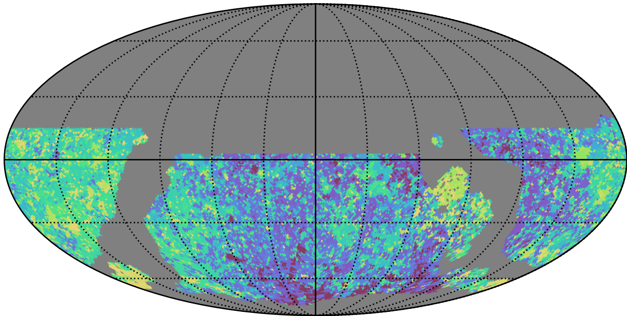
noroll_mjdp270_v3.4_10yrs WFD y band: Max Inter-Night Gap
