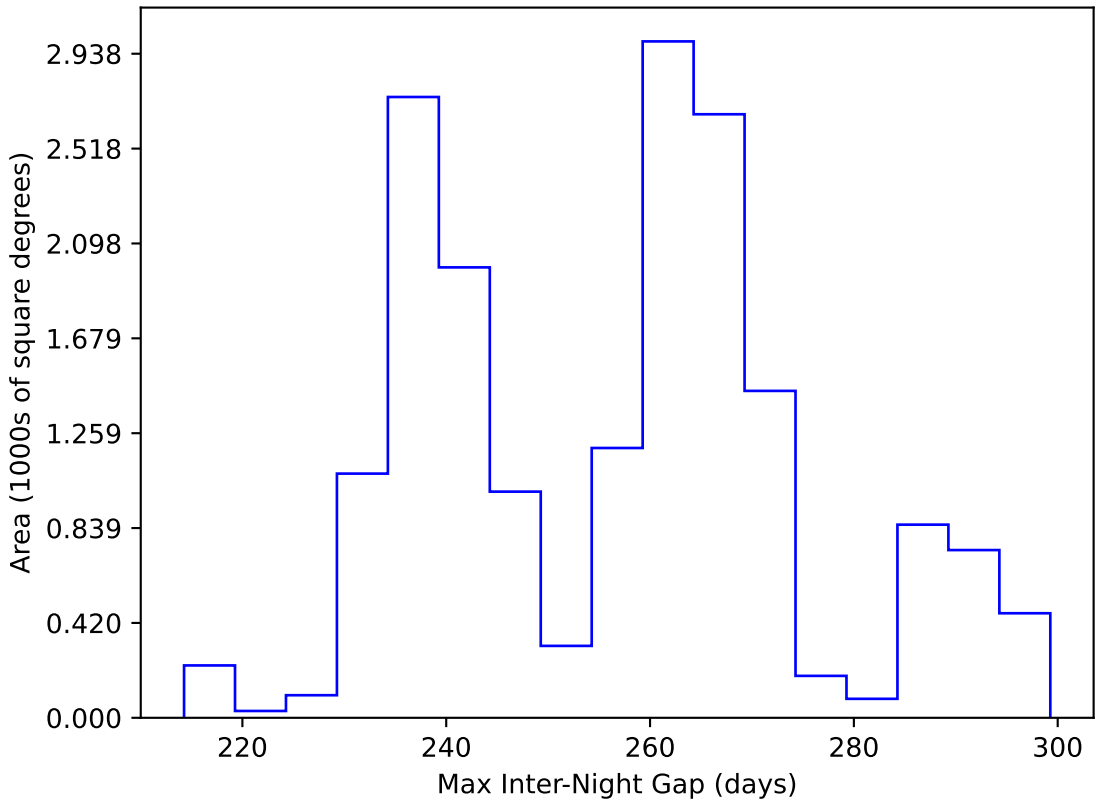
noroll_mjdp270_v3.4_10yrs WFD y band: Max Inter-Night Gap
