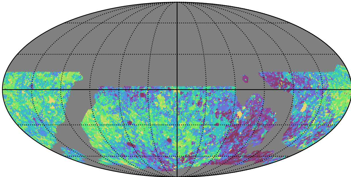
noroll_mjdp270_v3.4_10yrs WFD r band: Max Inter-Night Gap
