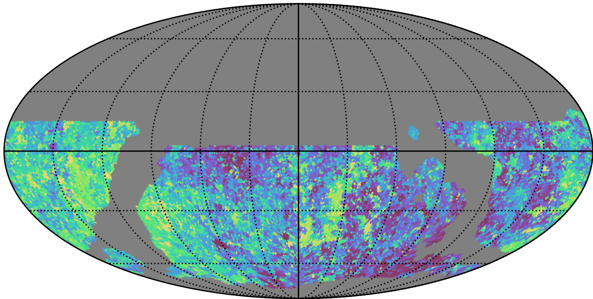
noroll_mjdp270_v3.4_10yrs WFD i band: Max Inter-Night Gap
