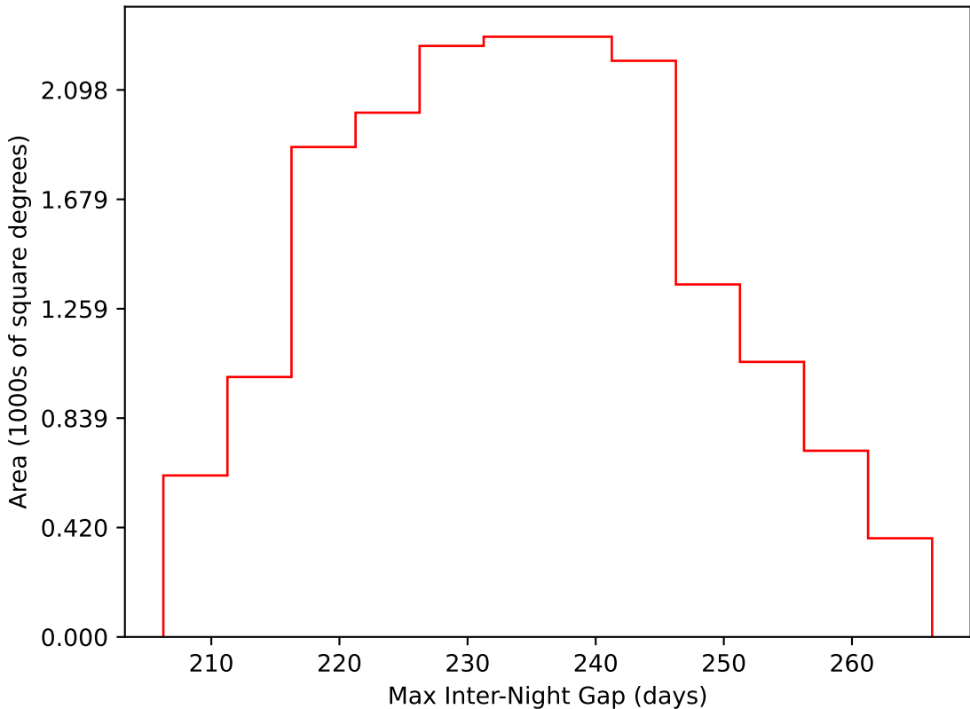
noroll_mjdp270_v3.4_10yrs WFD i band: Max Inter-Night Gap
