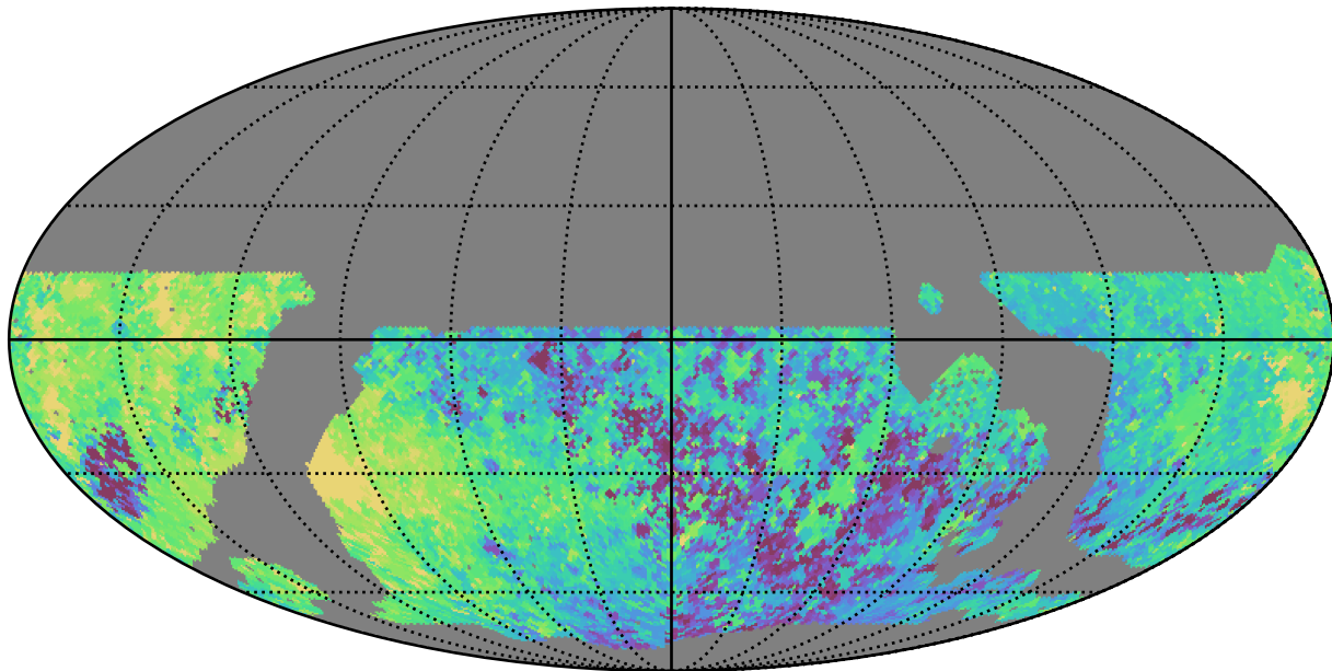
noroll_mjdp270_v3.4_10yrs WFD all bands: Max Inter-Night Gap
