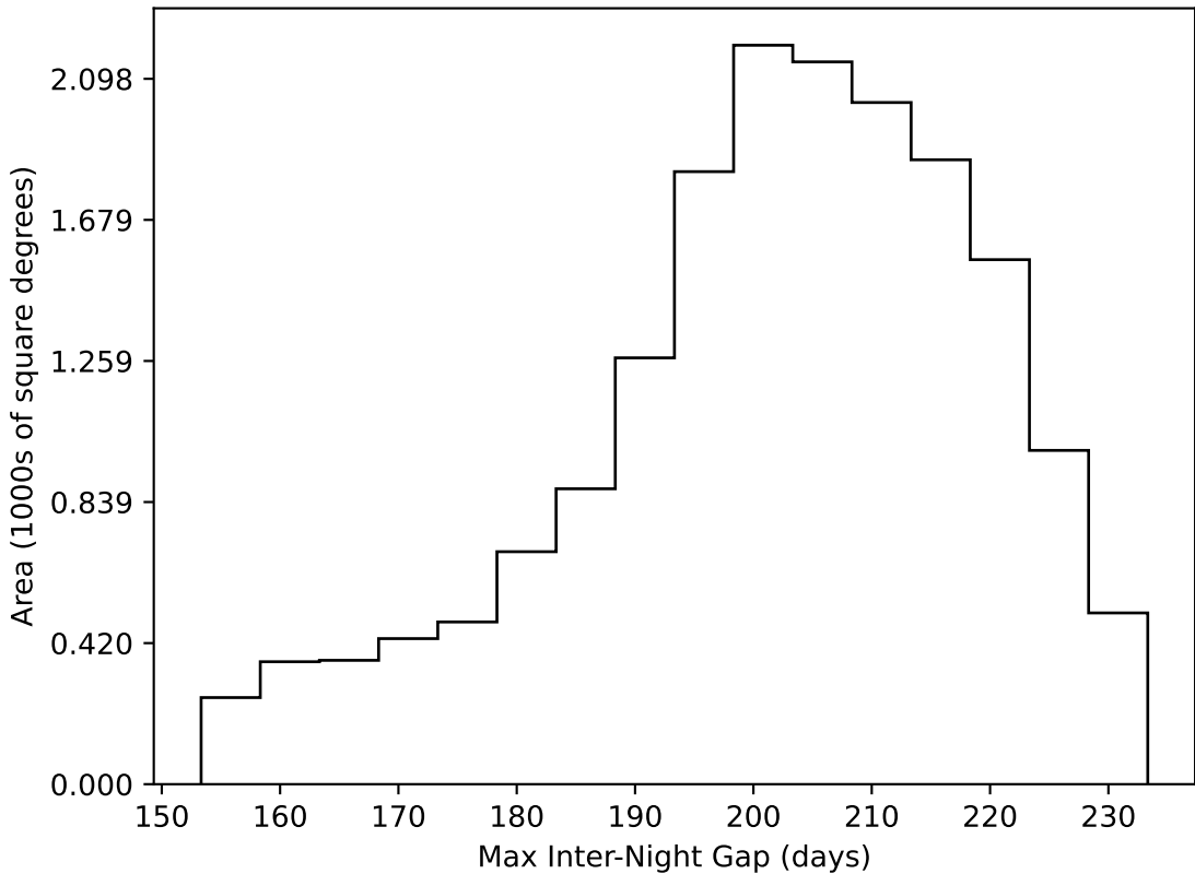
noroll_mjdp270_v3.4_10yrs WFD all bands: Max Inter-Night Gap
