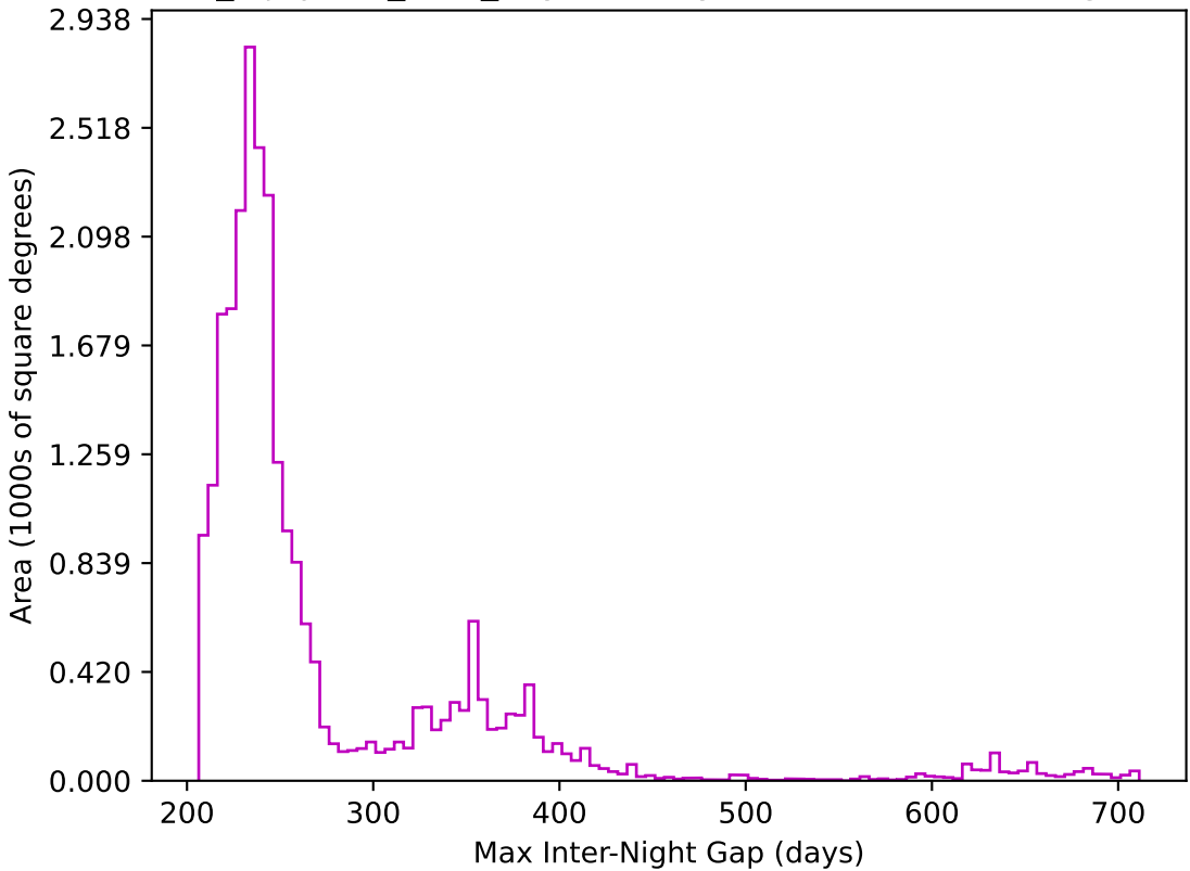
noroll_mjdp270_v3.4_10yrs All sky z band: Max Inter-Night Gap
