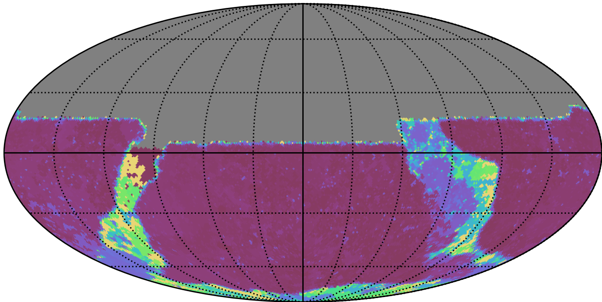
noroll_mjdp270_v3.4_10yrs All sky u band: Max Inter-Night Gap
