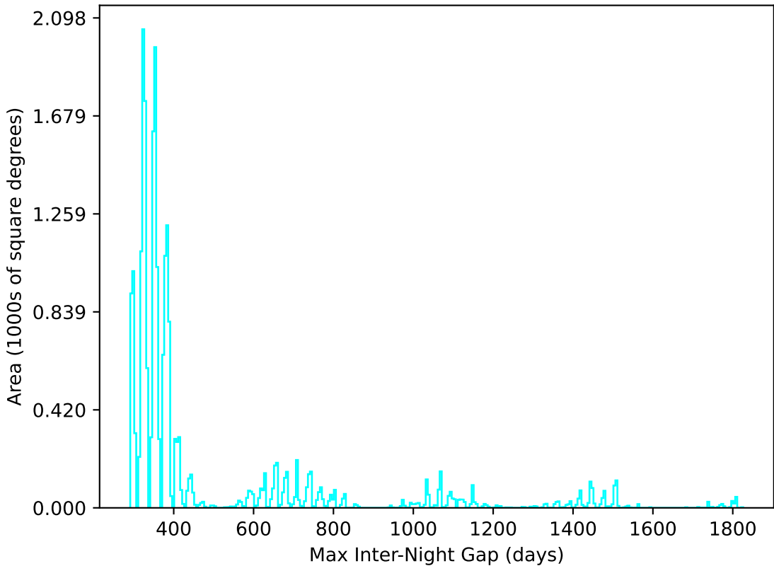
noroll_mjdp270_v3.4_10yrs All sky u band: Max Inter-Night Gap
