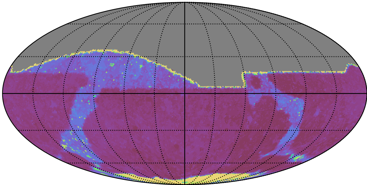
noroll_mjdp270_v3.4_10yrs All sky r band: Max Inter-Night Gap
