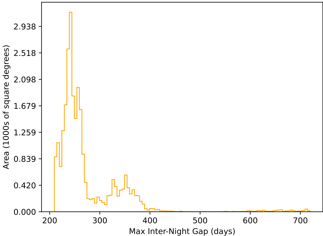
noroll_mjdp270_v3.4_10yrs All sky r band: Max Inter-Night Gap
