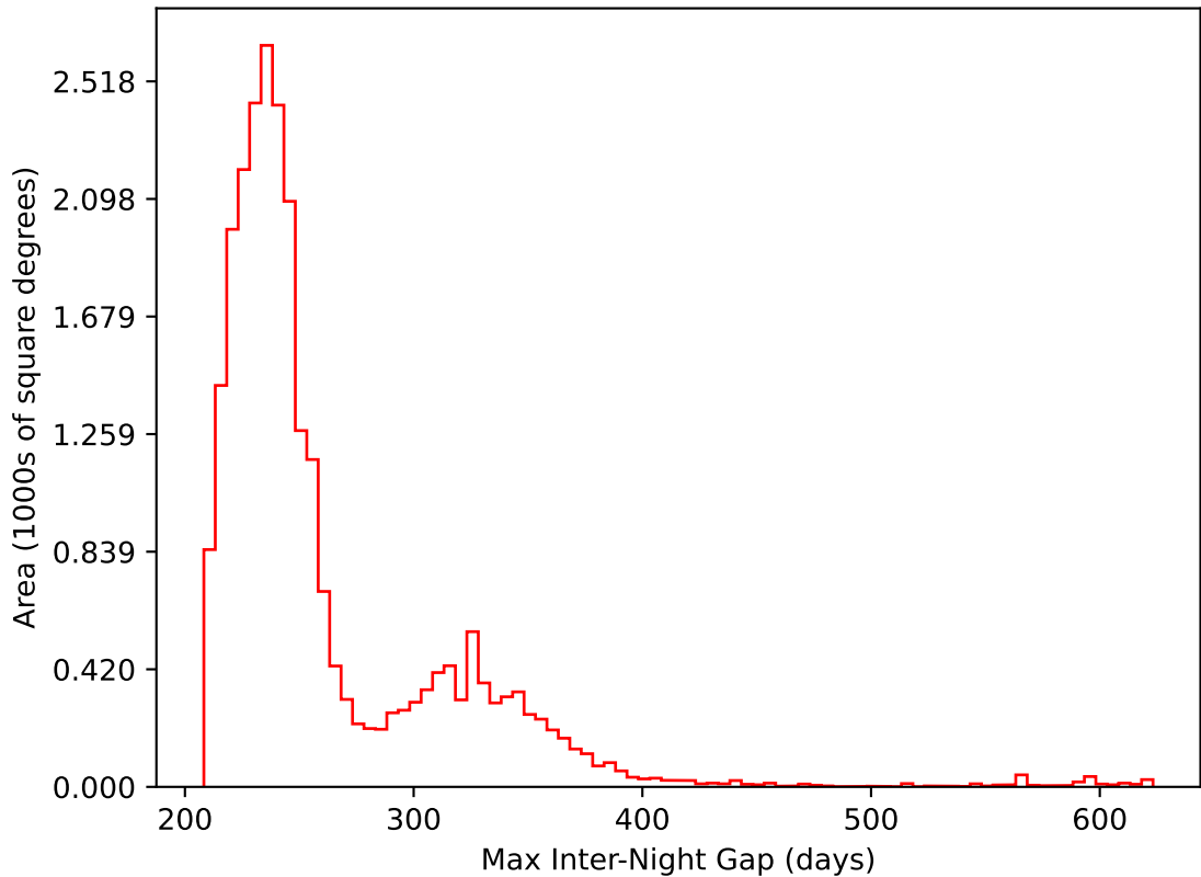
noroll_mjdp270_v3.4_10yrs All sky i band: Max Inter-Night Gap
