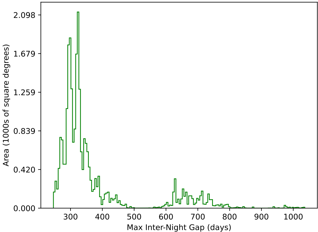
noroll_mjdp270_v3.4_10yrs All sky g band: Max Inter-Night Gap
