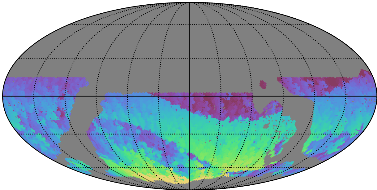
noroll_mjdp270_v3.4_10yrs WFD z band: Max HA
