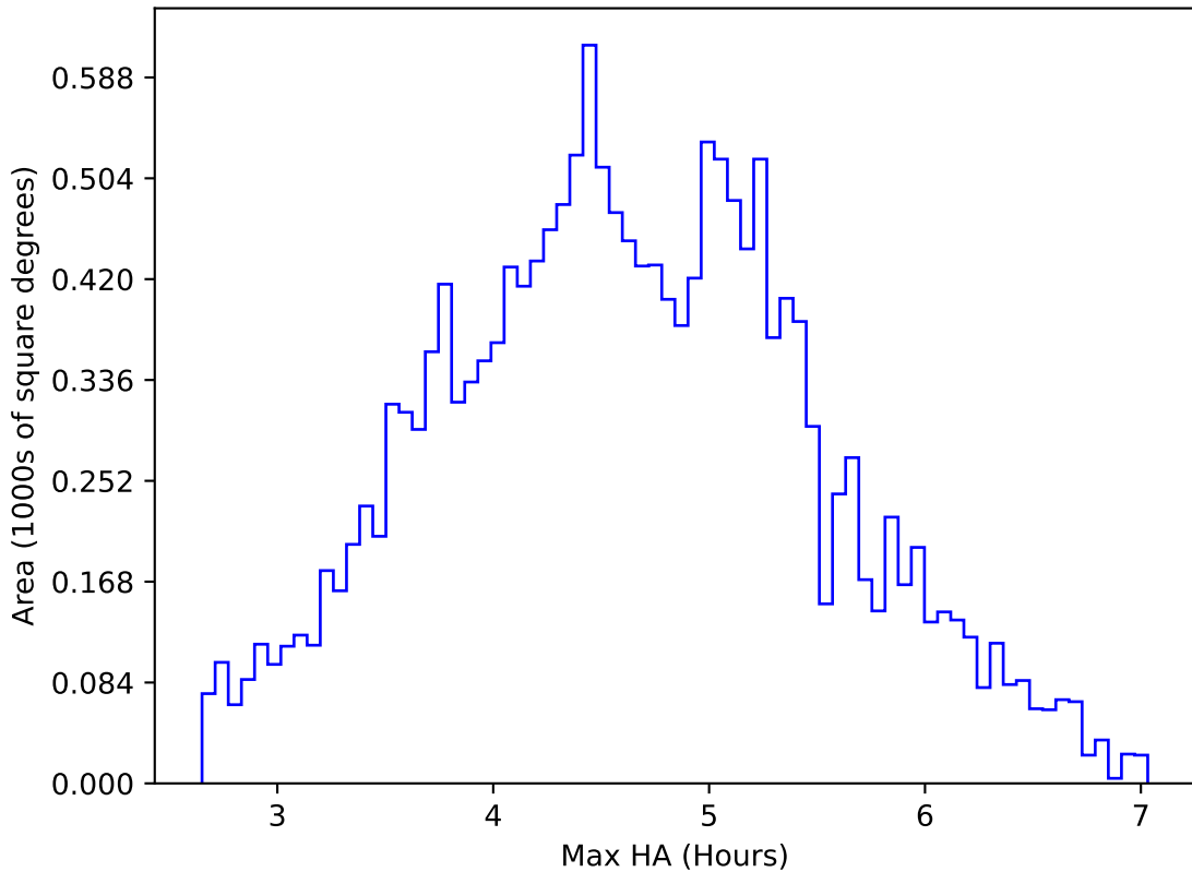
noroll_mjdp270_v3.4_10yrs WFD z band: Max HA
