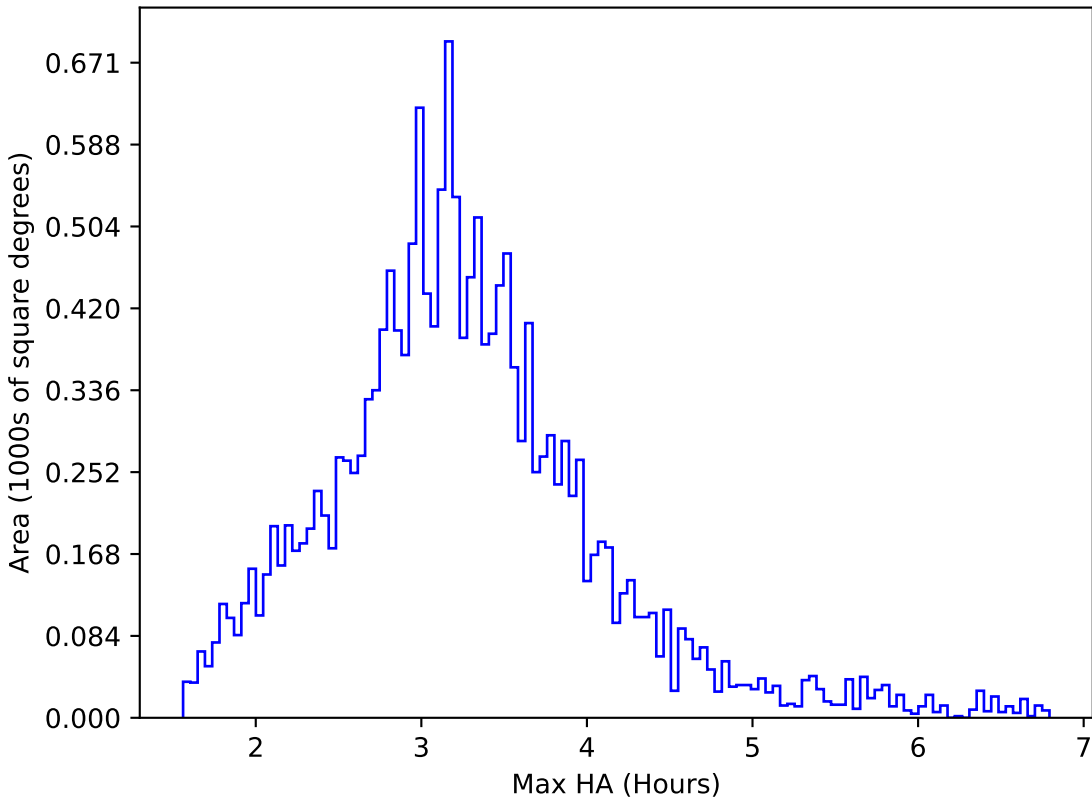
noroll_mjdp270_v3.4_10yrs WFD u band: Max HA
