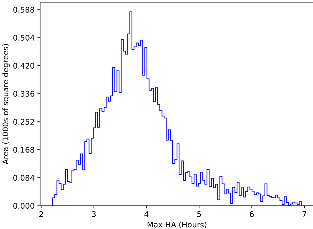
noroll_mjdp270_v3.4_10yrs WFD r band: Max HA
