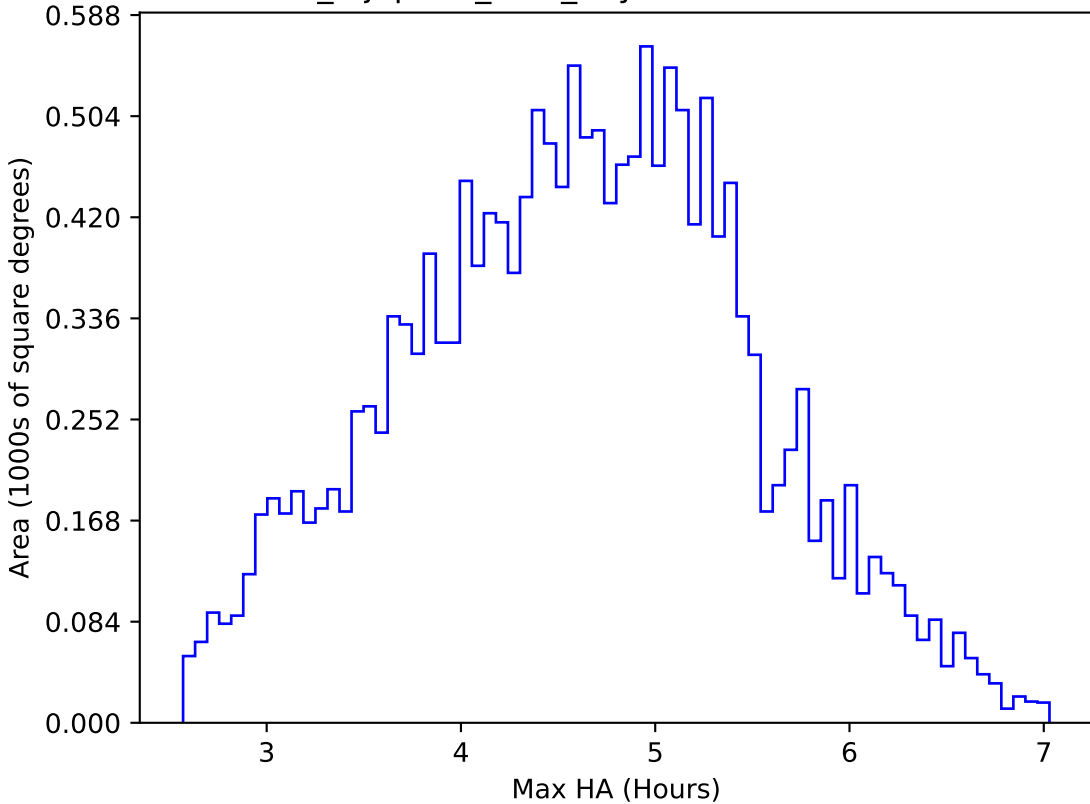
noroll_mjdp270_v3.4_10yrs WFD i band: Max HA
