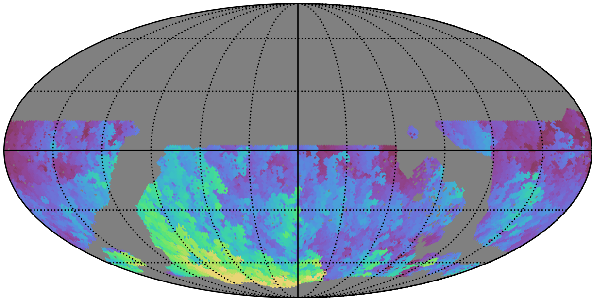
noroll_mjdp270_v3.4_10yrs WFD g band: Max HA
