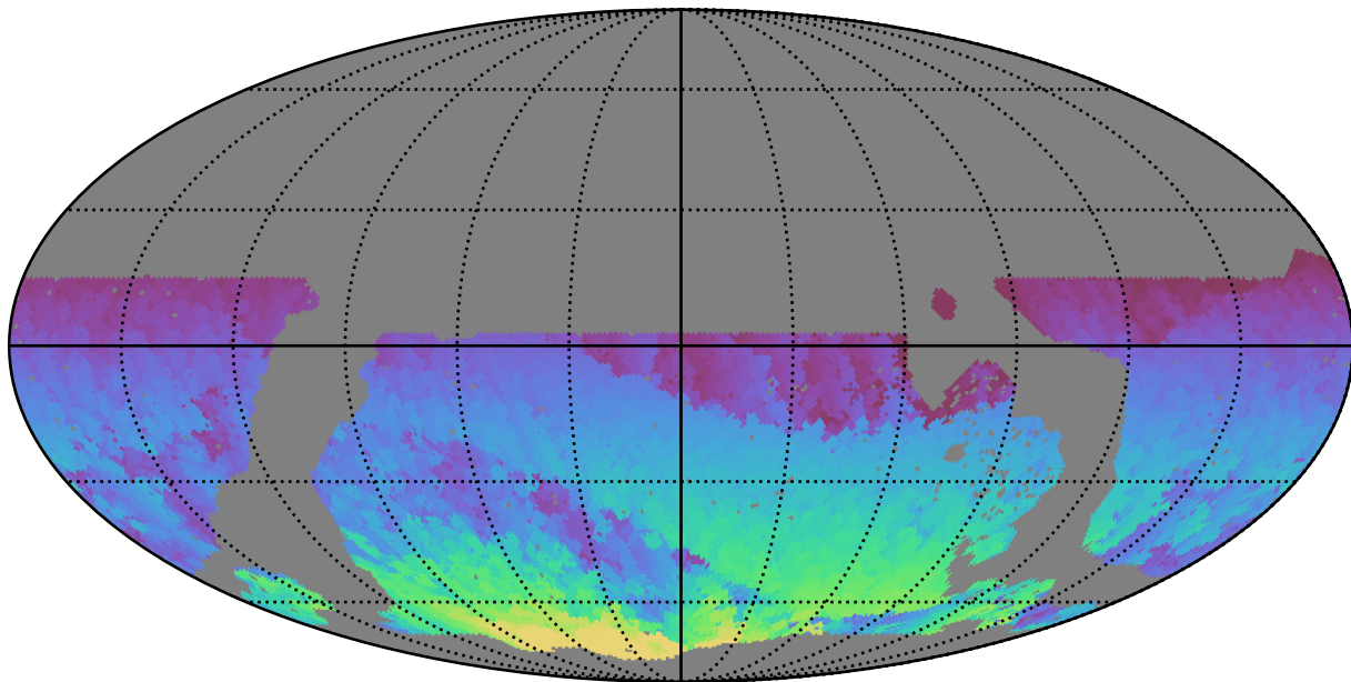
noroll_mjdp270_v3.4_10yrs WFD all bands: Max HA
