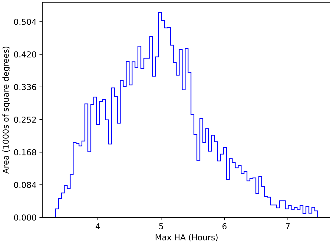
noroll_mjdp270_v3.4_10yrs WFD all bands: Max HA
