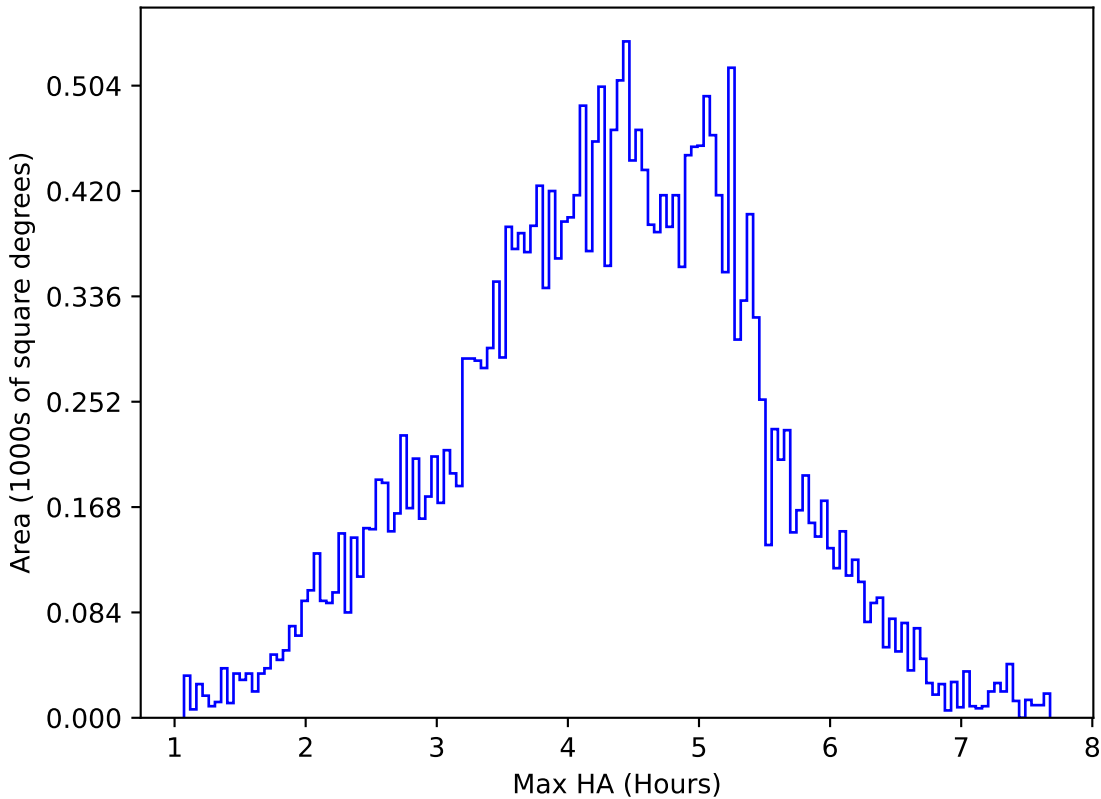
noroll_mjdp270_v3.4_10yrs All sky z band: Max HA
