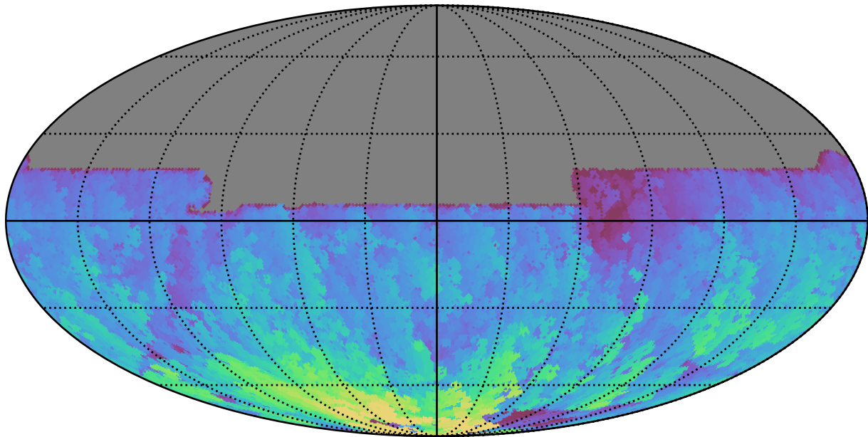
noroll_mjdp270_v3.4_10yrs All sky y band: Max HA
