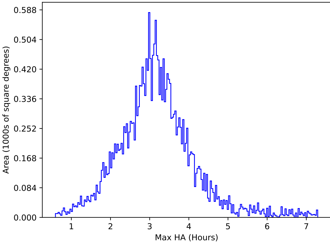
noroll_mjdp270_v3.4_10yrs All sky u band: Max HA
