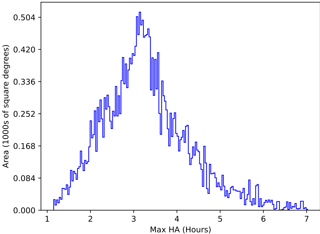
noroll_mjdp270_v3.4_10yrs All sky g band: Max HA
